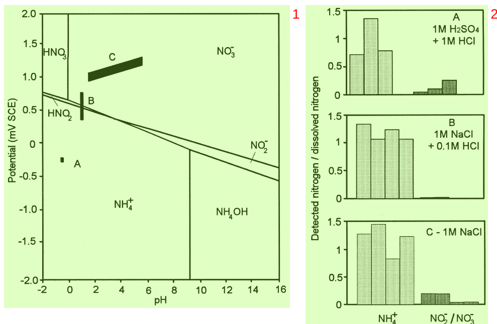
Fig. 12. Pourbaix diagram [74] for nitrogen showing potential–pH regions in which solution analyses were performed for K3 and proportion of the dissolved nitrogen (from weight loss measurements) analysed as \text{NH}_4^+ or \text{NO}_2^-/\text{NO}_3^- . Dissolution was by active corrosion in A, pitting corrosion in B and transpassive corrosion in C.
