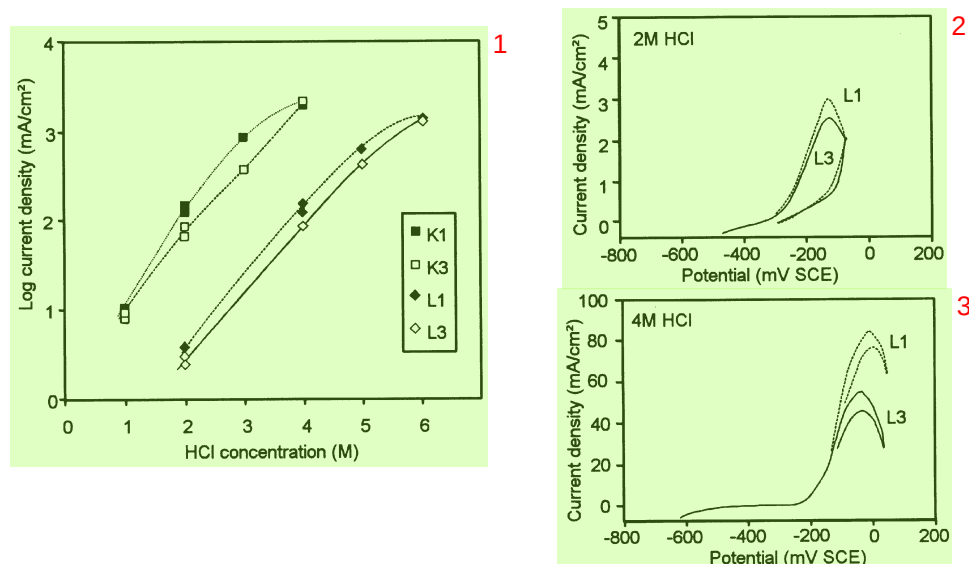
Fig. 7. (a) Peak anodic current density in HCl at 10 mV/s. The effect of nitrogen in decreasing the peak anodic current density is most pronounced at intermediate HCl concentrations. (b) Effect of potential scan reversal on polarisation curves. In 2 M HCl, passivation proceeds when the potential is decreased; in 4 M HCl, the passivation process is reversed for both L1 and L3.
