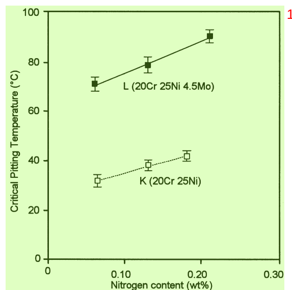
Fig. 1. Critical pitting temperature in 0.2 M NaCl at +600 mV SCE. Mo–N synergy is apparent from the steeper gradient for the L series with 4.5% Mo ( 144^{\circ}\text{C}/\% \text{N} ) compared to the Mo-free K series ( 86^{\circ}\text{C}/\% \text{N} ). Error bars denote maximum and minimum values.
