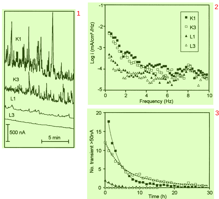
Fig. 6. Current transients measured during passive current density measurements in 0.5 M NaCl, pH 3 at +150 mV SCE. (a) Current-time trace after 30 min. (b) Current noise after same time. (c) Number of activations (> 50 nA).
