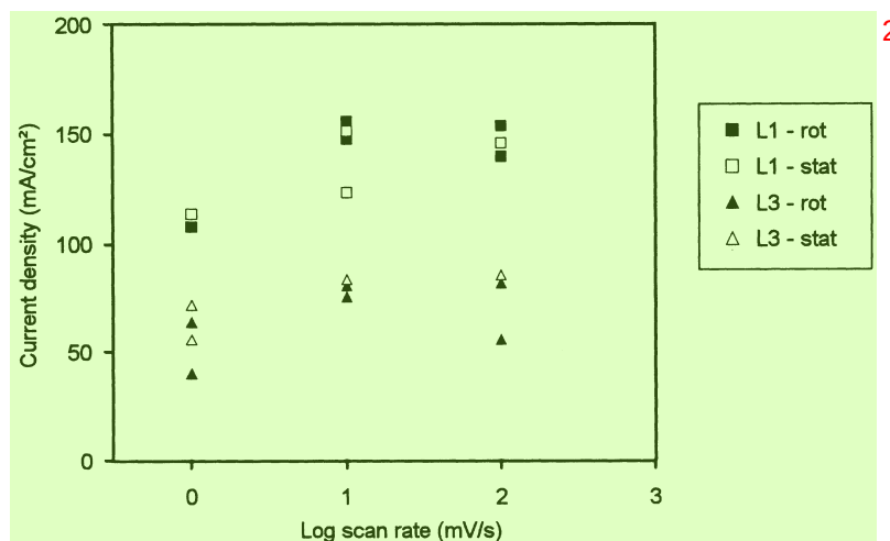
Fig. 8. Peak anodic current density for L1 and L3 in 4 M HCl at various potential scan rates and rotation speeds. 'rot' denotes 4000 rpm.
