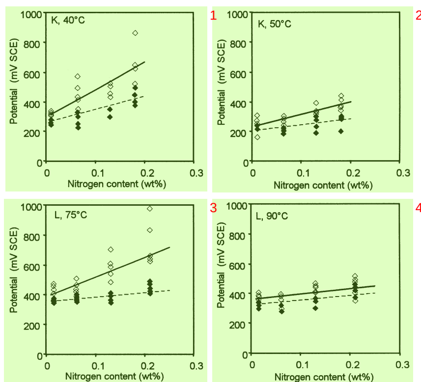
Fig. 3. Pitting potential measurements at various temperatures showing the final breakdown potential E_b (open points) and the potential E_{mit} at which the first repassivating pits were observed (solid points).
